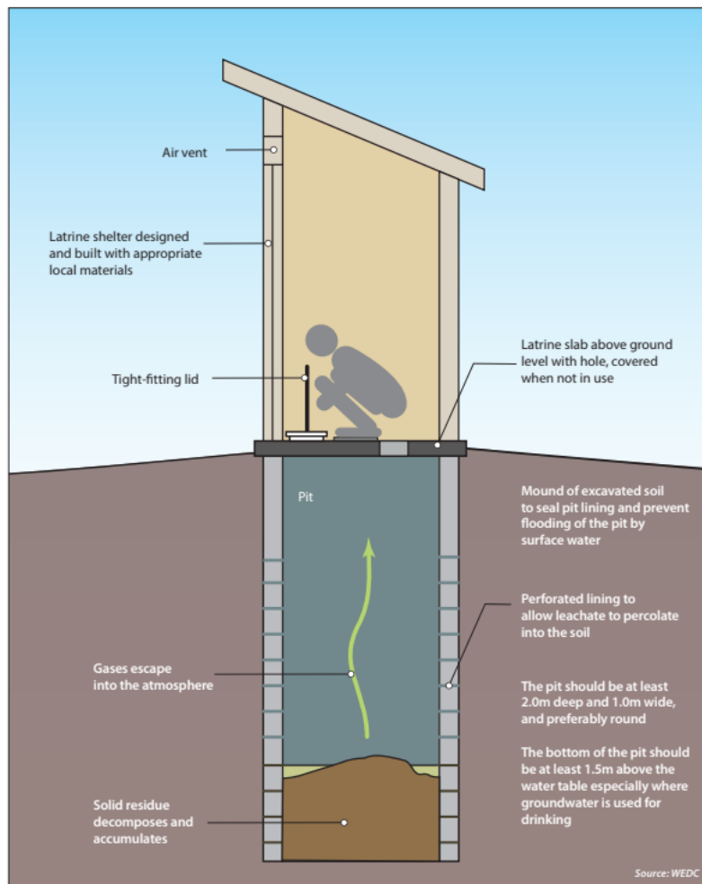
A single pit latrine. (Source: WHO: Guidelines on Sanitation and Health 2018)
