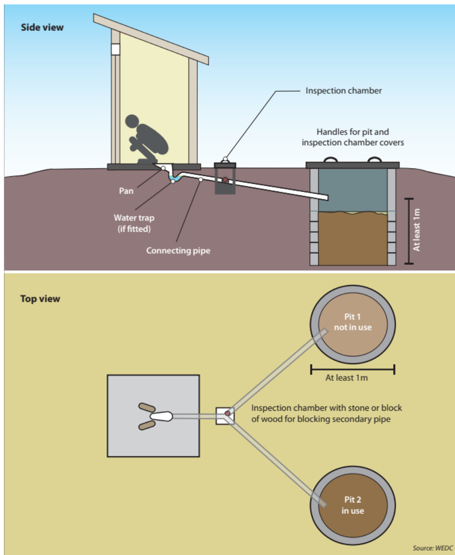
A twin-pit pour flush latrine. (Source: WHO: Guidelines on Sanitation and Health 2018)
