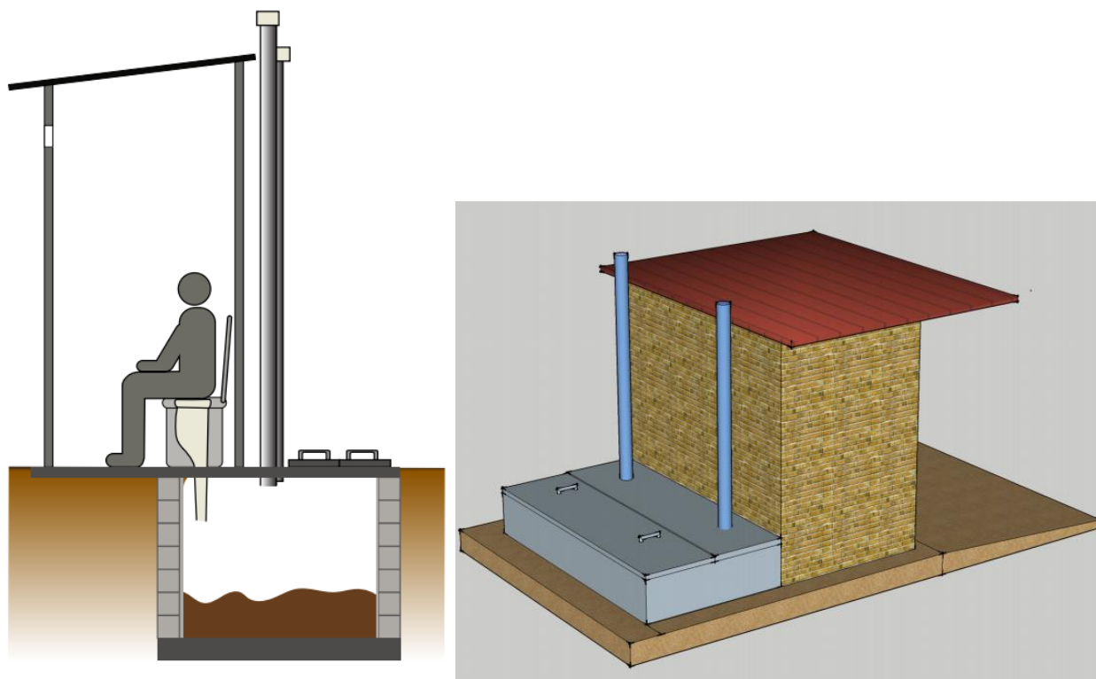
Two-dimensional view of KVIP (left) and back view of KVIP (right) (Source: UNICEF: Latrine Technology Manual)
