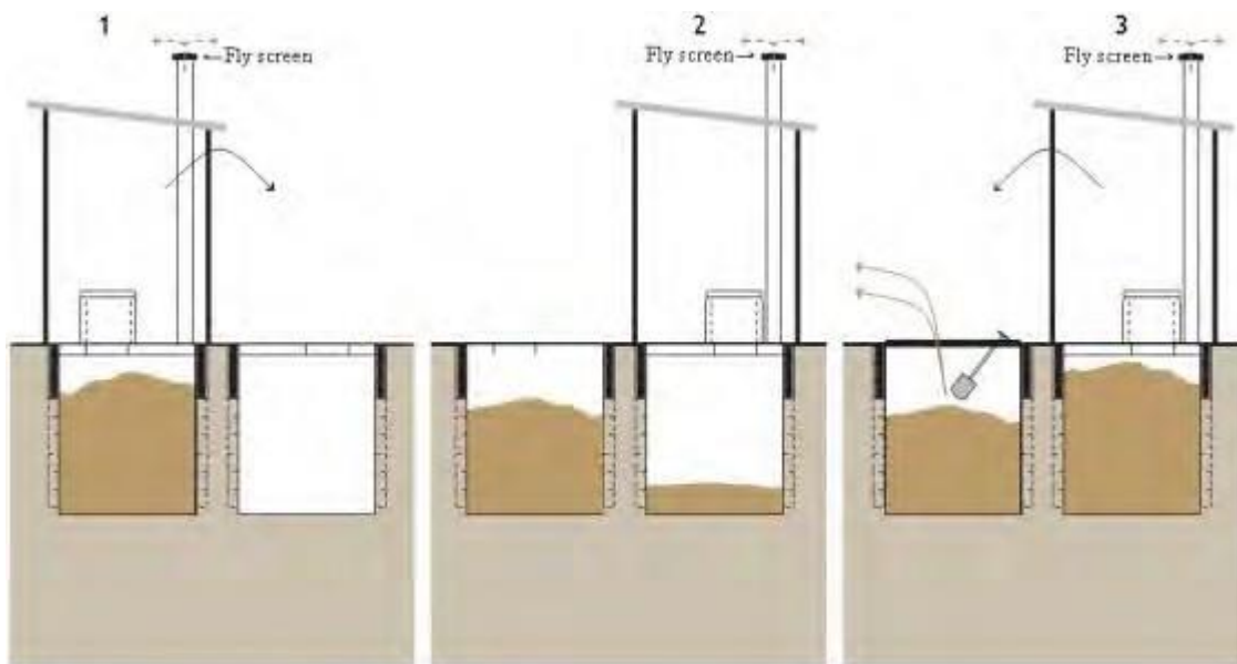
Functional staging of pits and superstructure. Source; SSWM – Stauffer/ Tilley et al - 2008).
