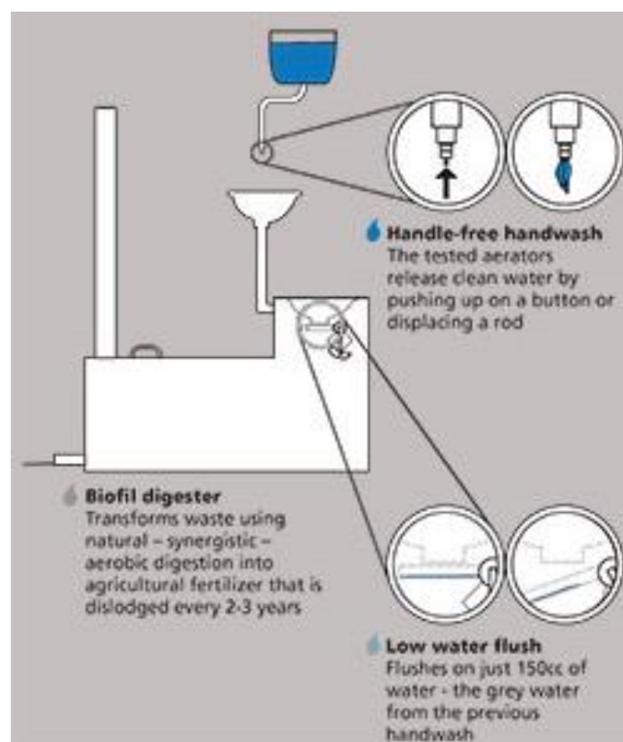
Micro-flush toilet design. (Source: Application of GSAP Microflush Toilets: a sustainable development approach to rural and peri-urban sanitation - Mecca, S.- et al 2013))
