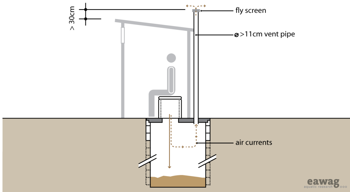
A single ventilated improved pit. (Source: Akvopedia: https://akvopedia.org/wiki/Single_Ventilated_Improved_Pit )
